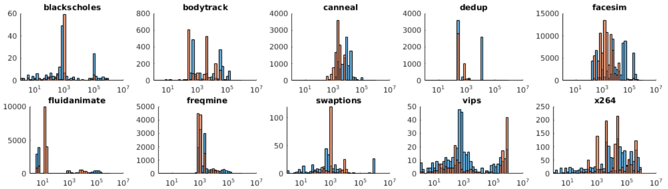
Fig. 3. This figure shows the page access histograms for the PARSEC 3.0 suite of benchmarks running the sims datasets. Blue indicates page accesses for reads, while red shows writes. The distribution of page accesses across an extremely large spectrum, as well as the different access patterns motivates the need for intelligent page placement when dealing with heterogeneous memories. streamcluster has been omitted due to space constraints.
